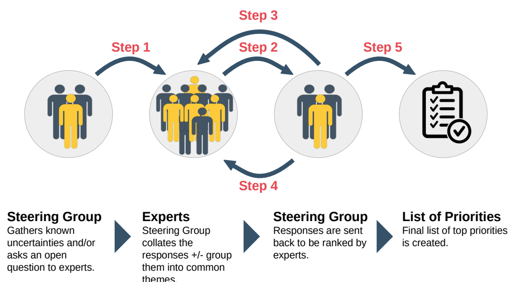
Figure 3: Delphi Technique
