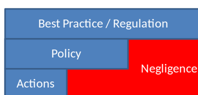
Figure 3: Negligence
