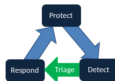
Figure 5: Incident Management
